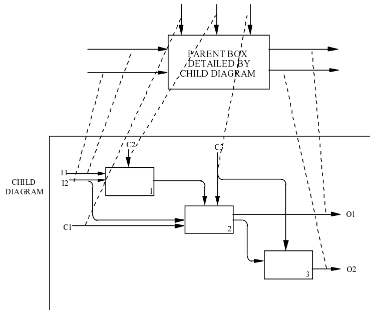
Figure 15. ICOM Codes and Changing Arrow Roles
