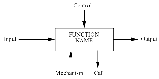
Figure 3. Arrow Positions and Roles
