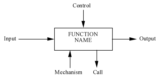
Figure A1. Function Box and Data/Objects Arrows
