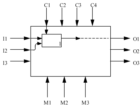
Figure B9. FEO representing detailing of multiple ICOMs
