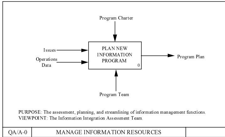
Figure 5. Example Top-level Diagram
