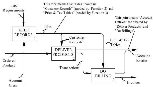
Figure 12. Connections Between Boxes
