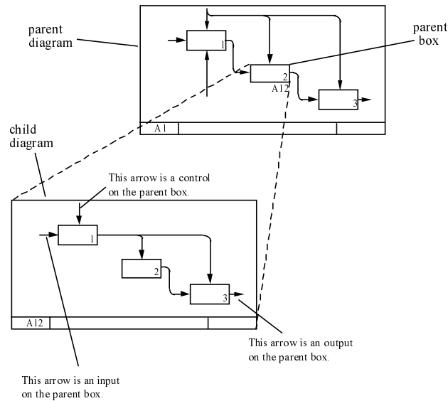
Figure 14. Boundary Arrow Correspondence
