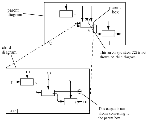
Figure 18. Example of Tunneled Arrows
