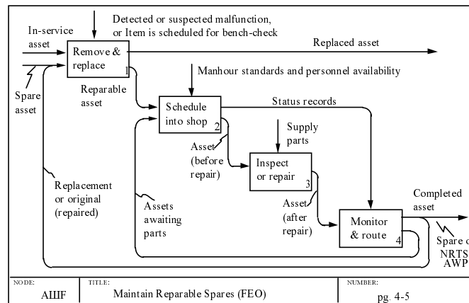
Figure B5. Example of Main Path
