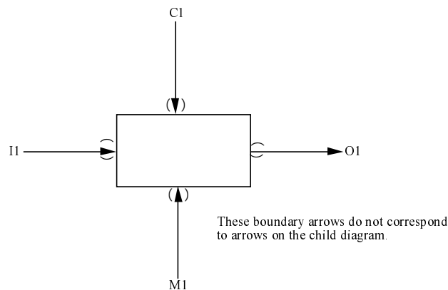
Figure 16. Arrows Tunneled at Connected End
