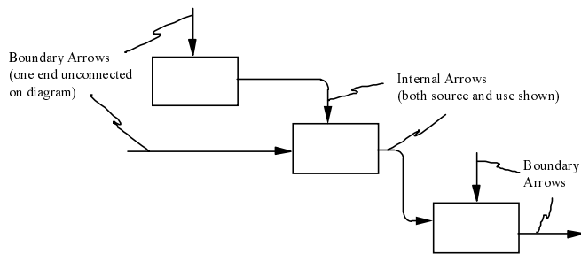
Figure 13. Boundary and Internal Arrows
