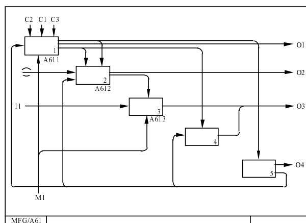
Figure 7. Detail Reference Expression Use
