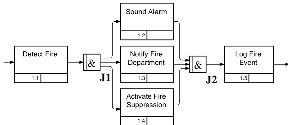
Figure 2-10. AND junctions.
